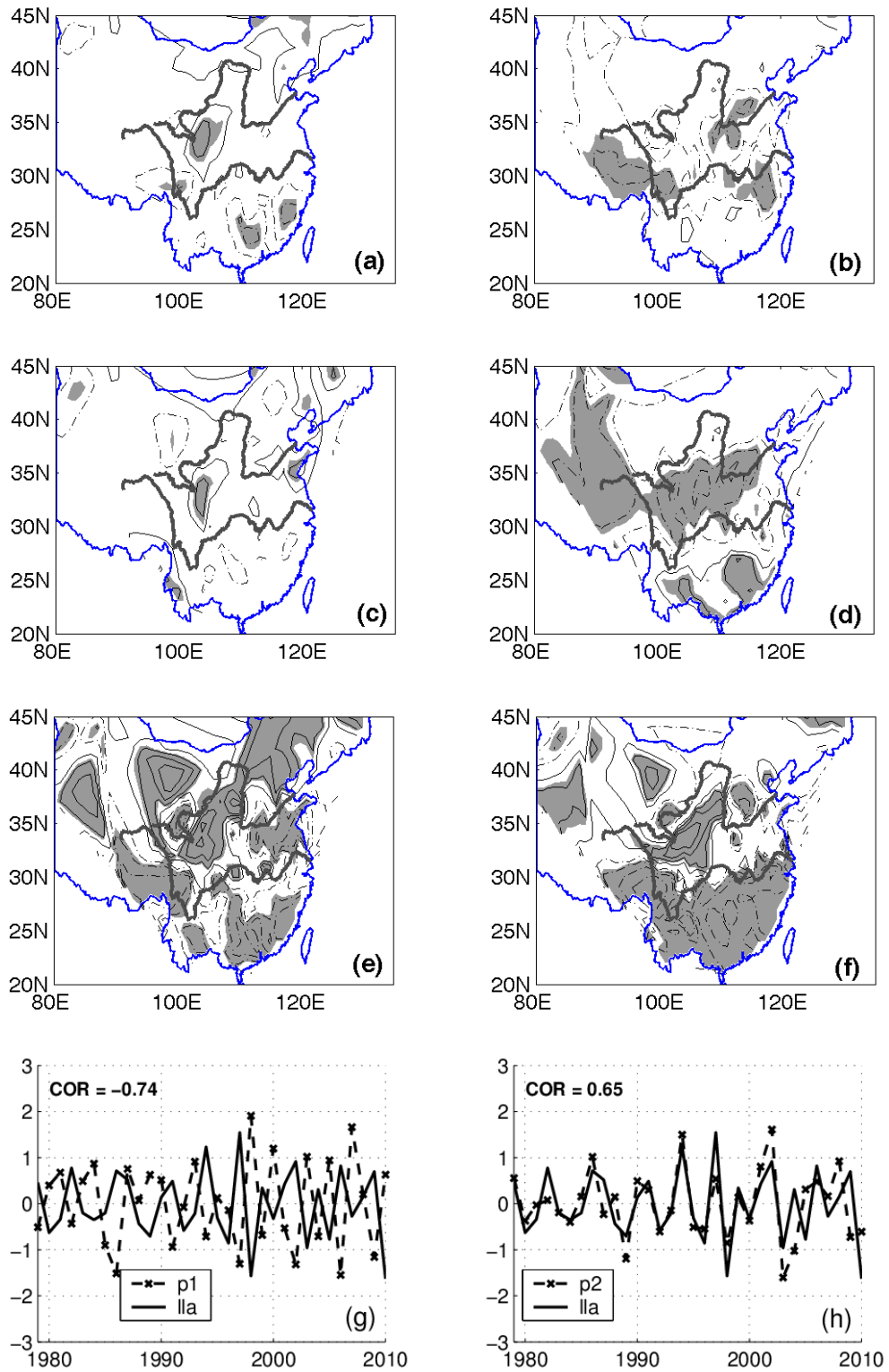
Fig. 3. Correlations between (a, b) the original data, (c, d) 9-year high-pass filtered data; (e, f) 9-year low-pass filtered data. LLS CEFs and LLA CEFs and 160-station summer rainfall observation data during the period 1979–2010. Shadings represent significant values at the 95% confidence level. Contour values are -0.6, -0.4, -0.2, 0.2, 0.4, 0.6 . The two thick curves show the location of the Yellow River and the Yangtze River. (g, h) The 9-year high-pass filtered regional mean rainfall indices and LLA CEFs during 1979–2010.
