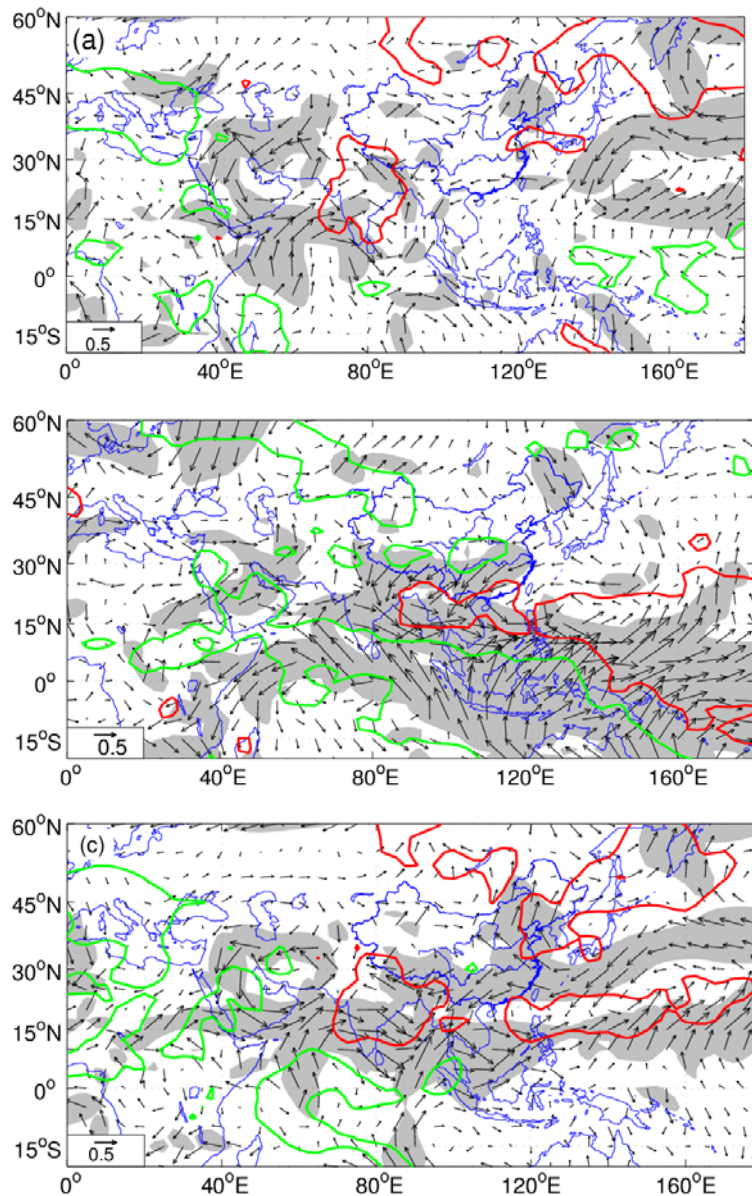
Fig. 4. Correlations between (a) the LLS CEFs, (b) LLA CEFs, (c) Somali low-level jet and the vertically integrated (300–1000 hPa) water vapor flux (arrows) and water vapor content for the 9-year high-pass filtered data. Contours represent significant correlations at 95% confidence level: red/green for positive/negative values. Shadings represent significant correlations for the wind field at 95% confidence level.
