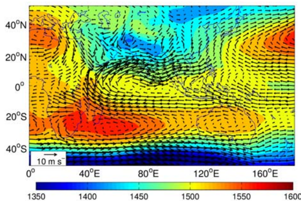
Fig. 1. Climatology of wind (arrows, units: \text{m s}^{-1} ) and geopotential height (shadings, units: gpm) at 850 hPa in summer during 1980–1999.
